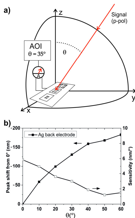
Figure 6. (a) Schematic illustration of the detector concept used for the detection of the AOI of incoming light. (b) Sensitivity and spectral shift of the resonance peak depending on the angle of incidence.
